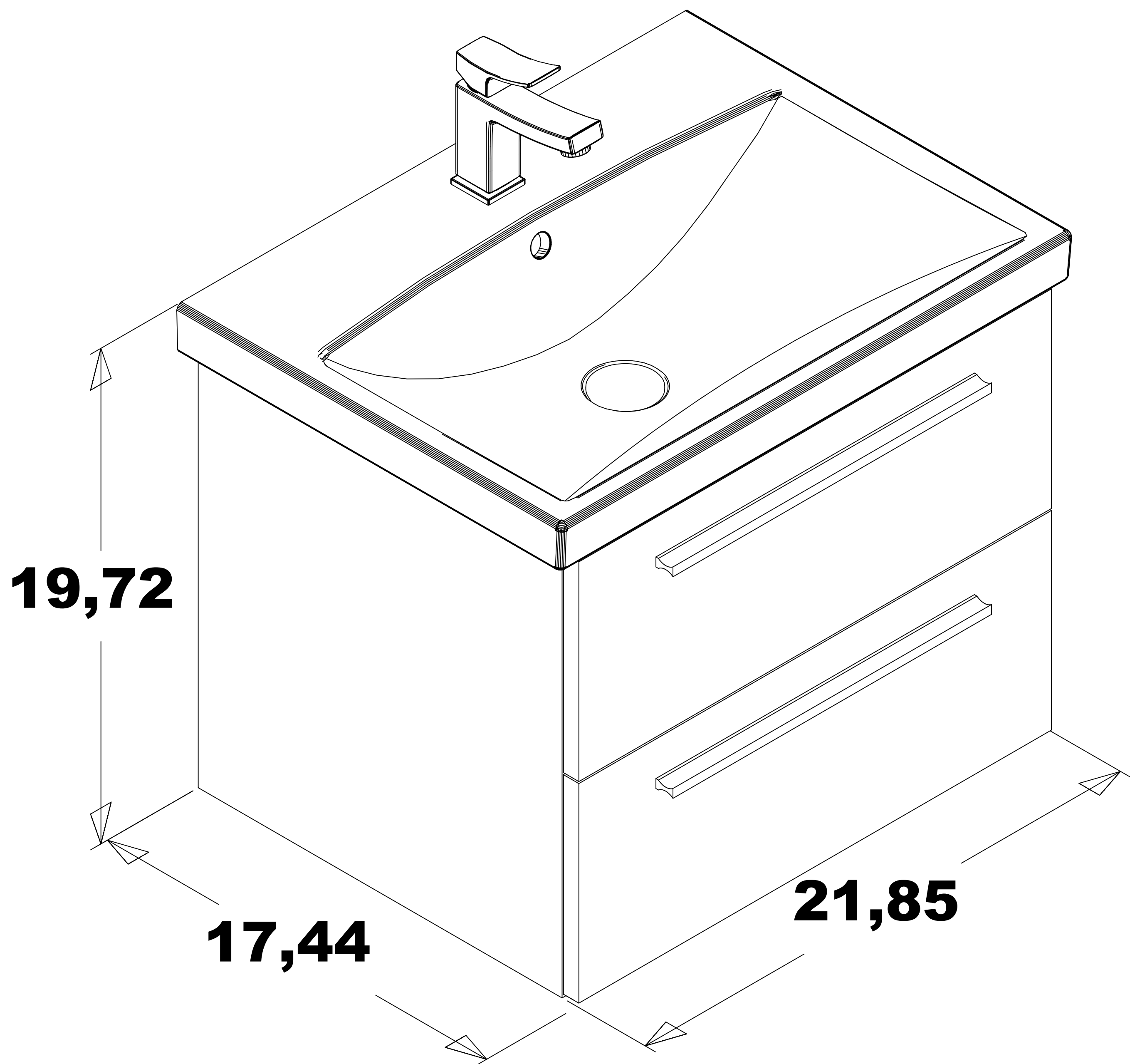
ISOMETRIC VIEW
