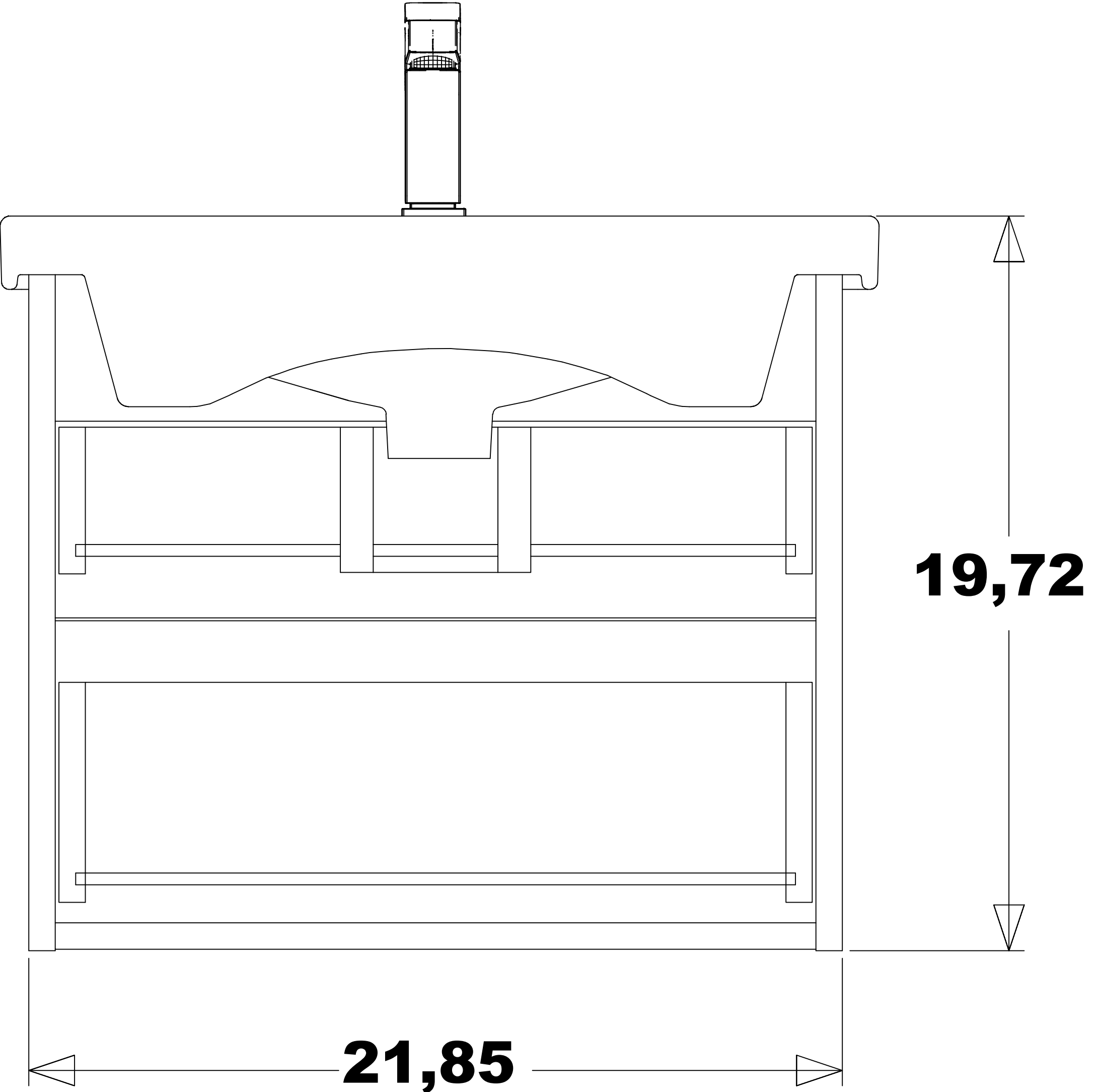
BACK VIEW
