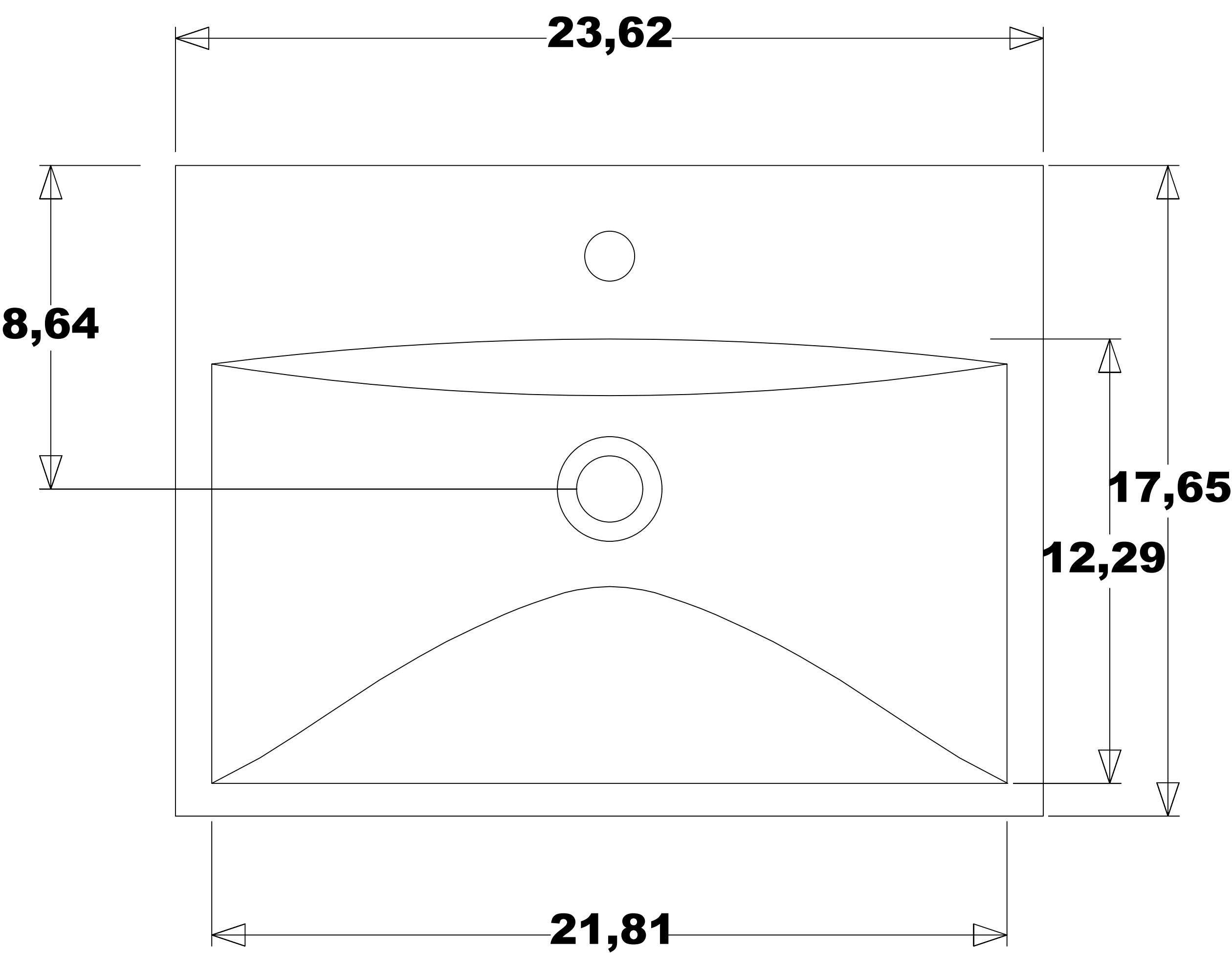
TOP VIEW
