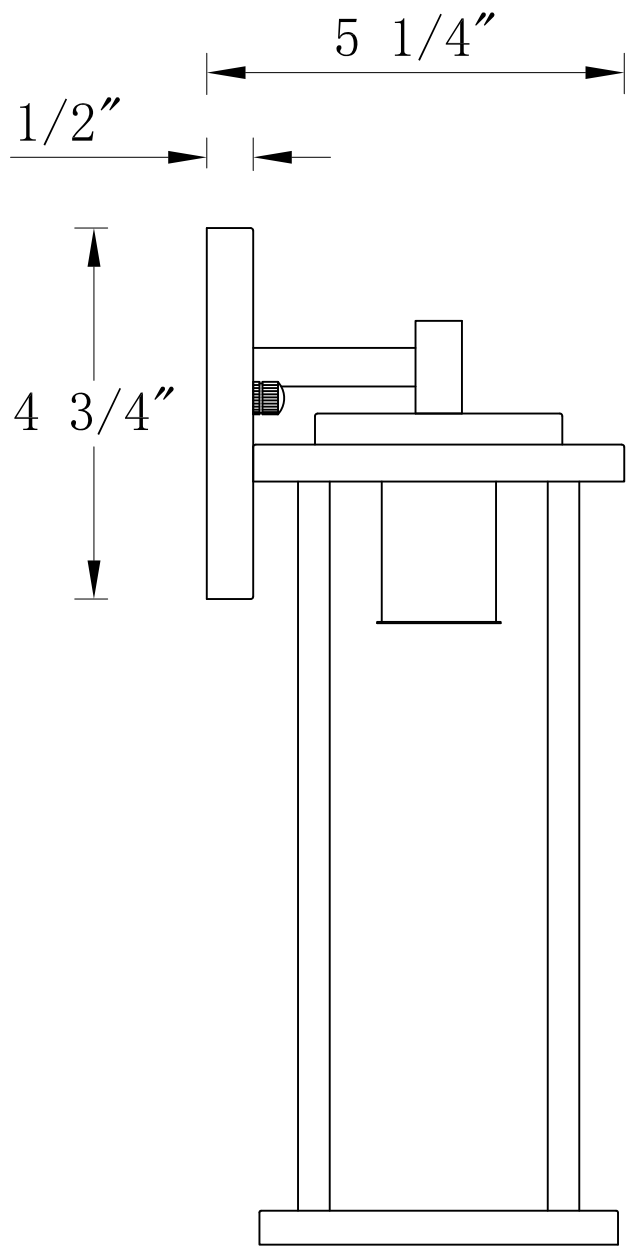
SIDE VIEW
