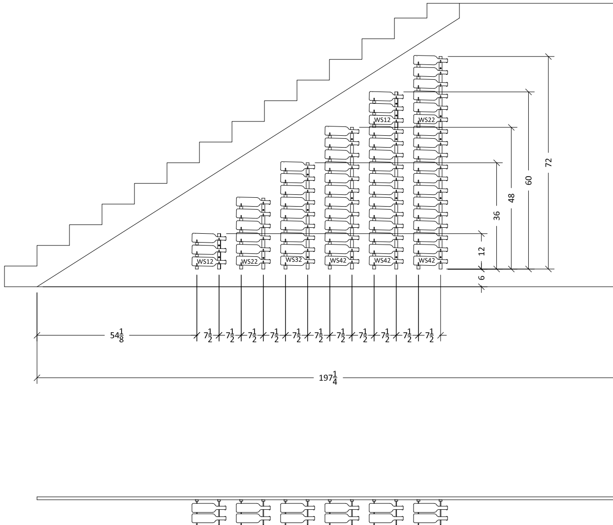
1 PLAN AND ELEVATION Scale: \frac{3}{8}" = 1'-0"
