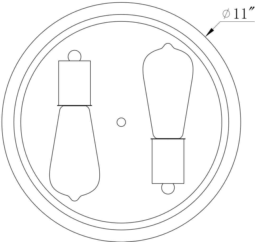
TOP VIEW
