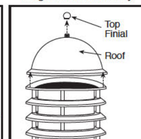
Figure 6 Louver Fixtures
