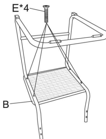
STEP 2. All bolts/screws are lined up and inserted into the holes, attach seat part(B) to the metal unit part (C) and part(D) assembled as shown, secure it well by using bolt(E) and wrench (F).
