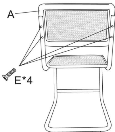
STEP 3. All bolts/screws are lined up and inserted into the holes, attach back part(A) to the metal unit part(C) and part(D) assembled as shown, secure it well by using bolt(E) and wrench(F)..
