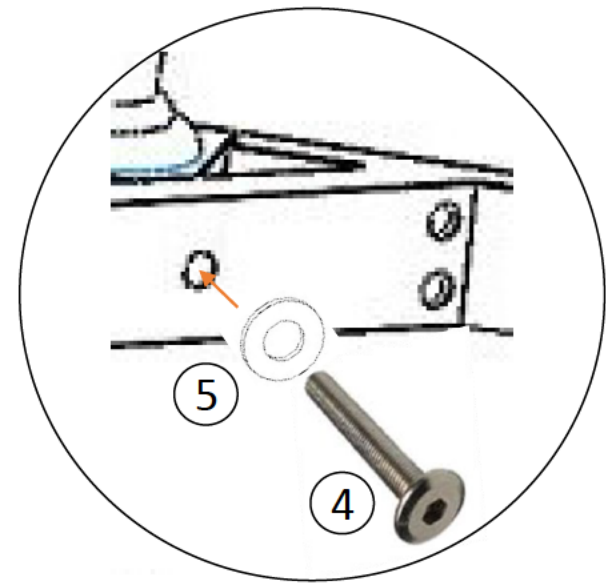
DETAIL X
