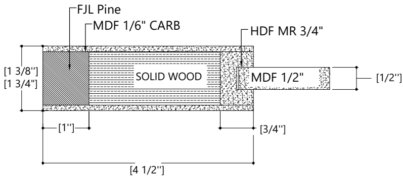
Section B - B ( Stile )
