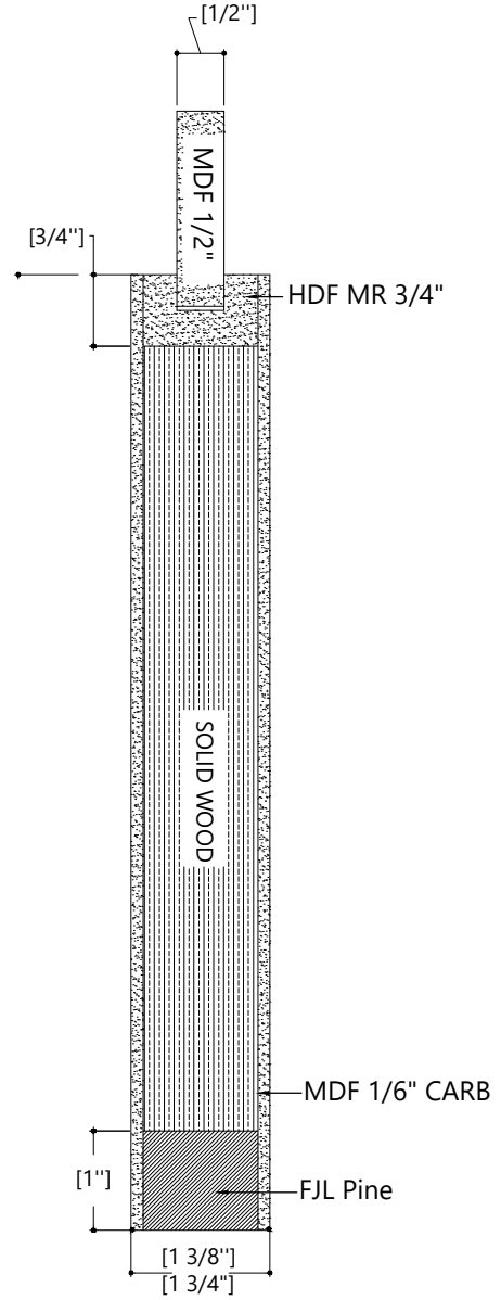
Section C - C ( Bottom Rail )
