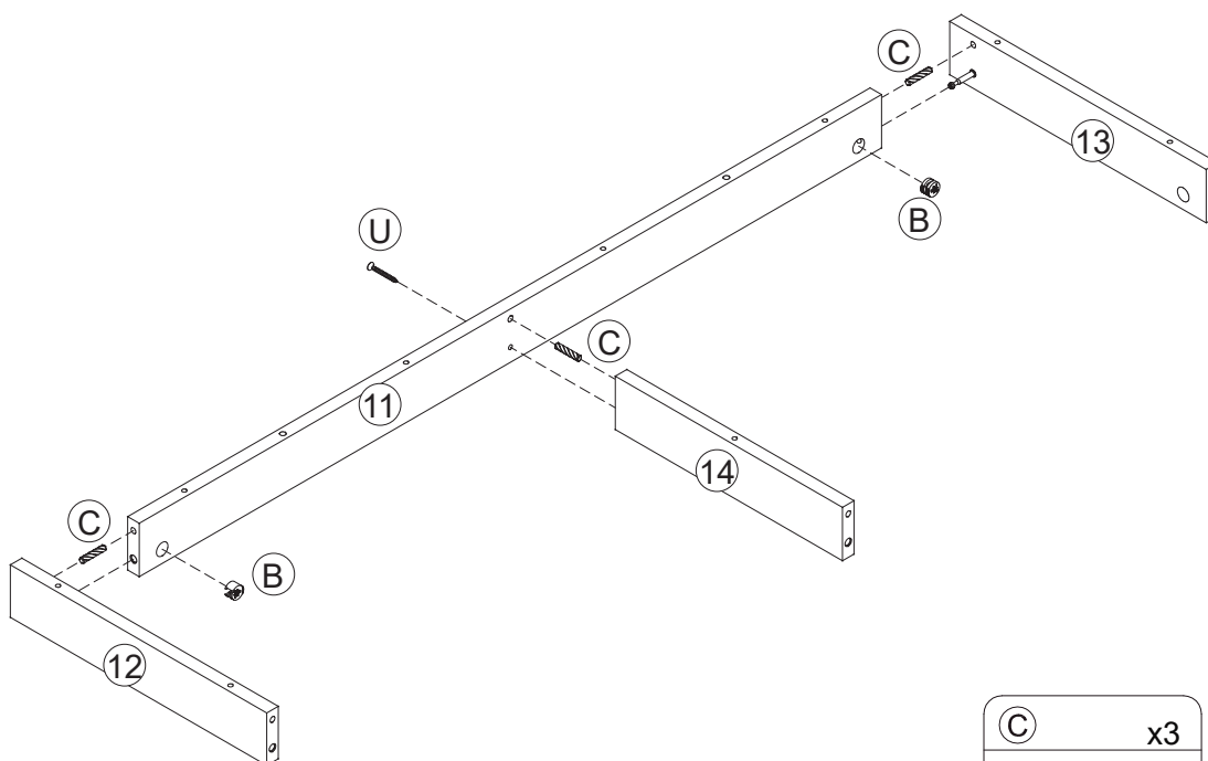
Cam Lock Fastening System
