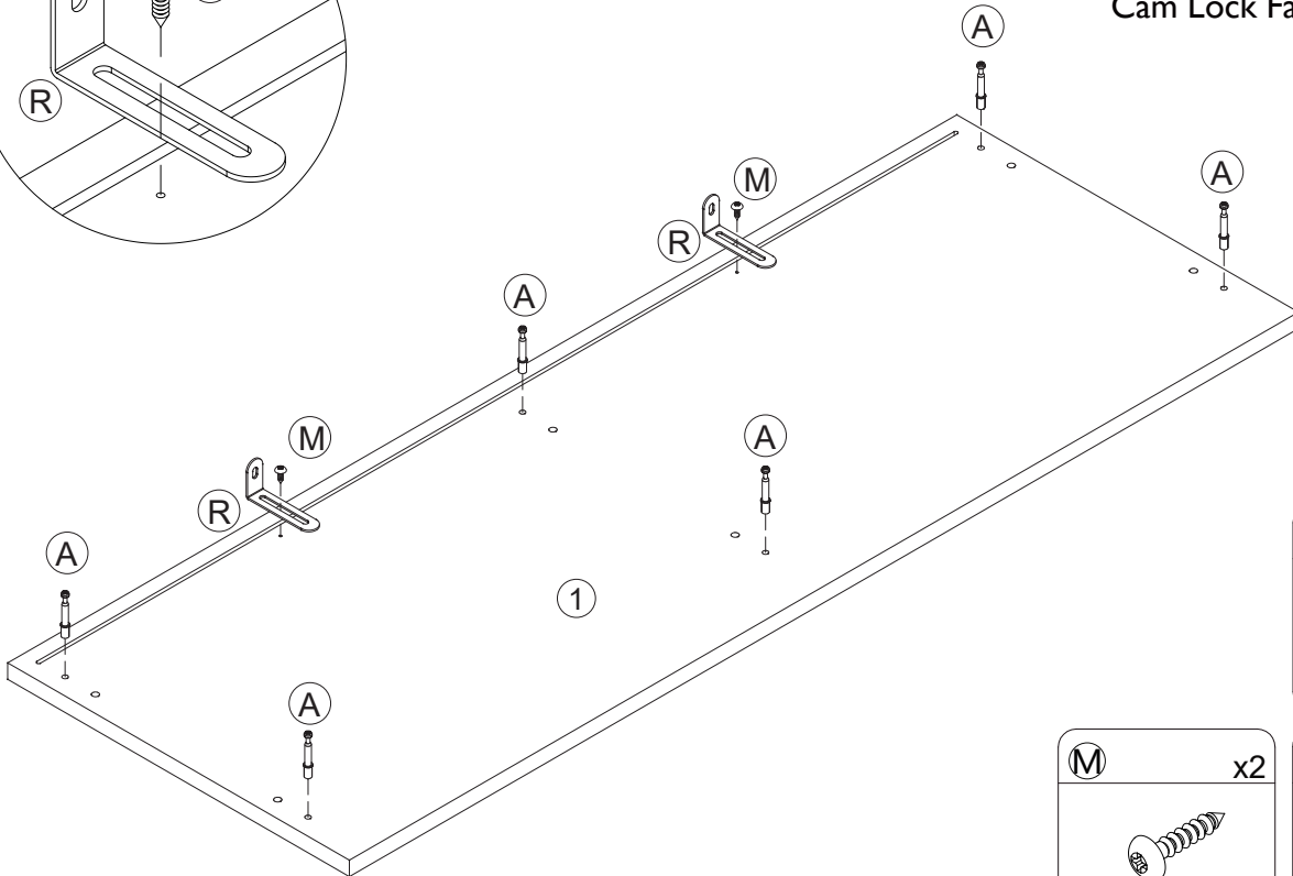
Cam Lock Fastening System
