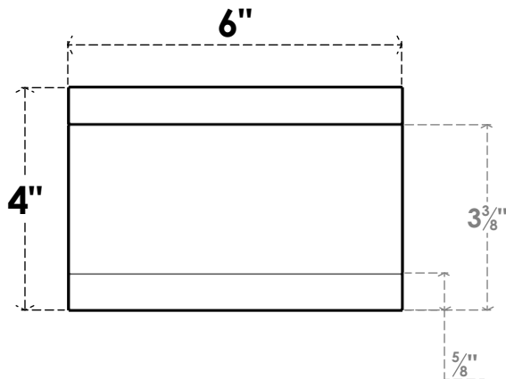
FRONT PROFILE
