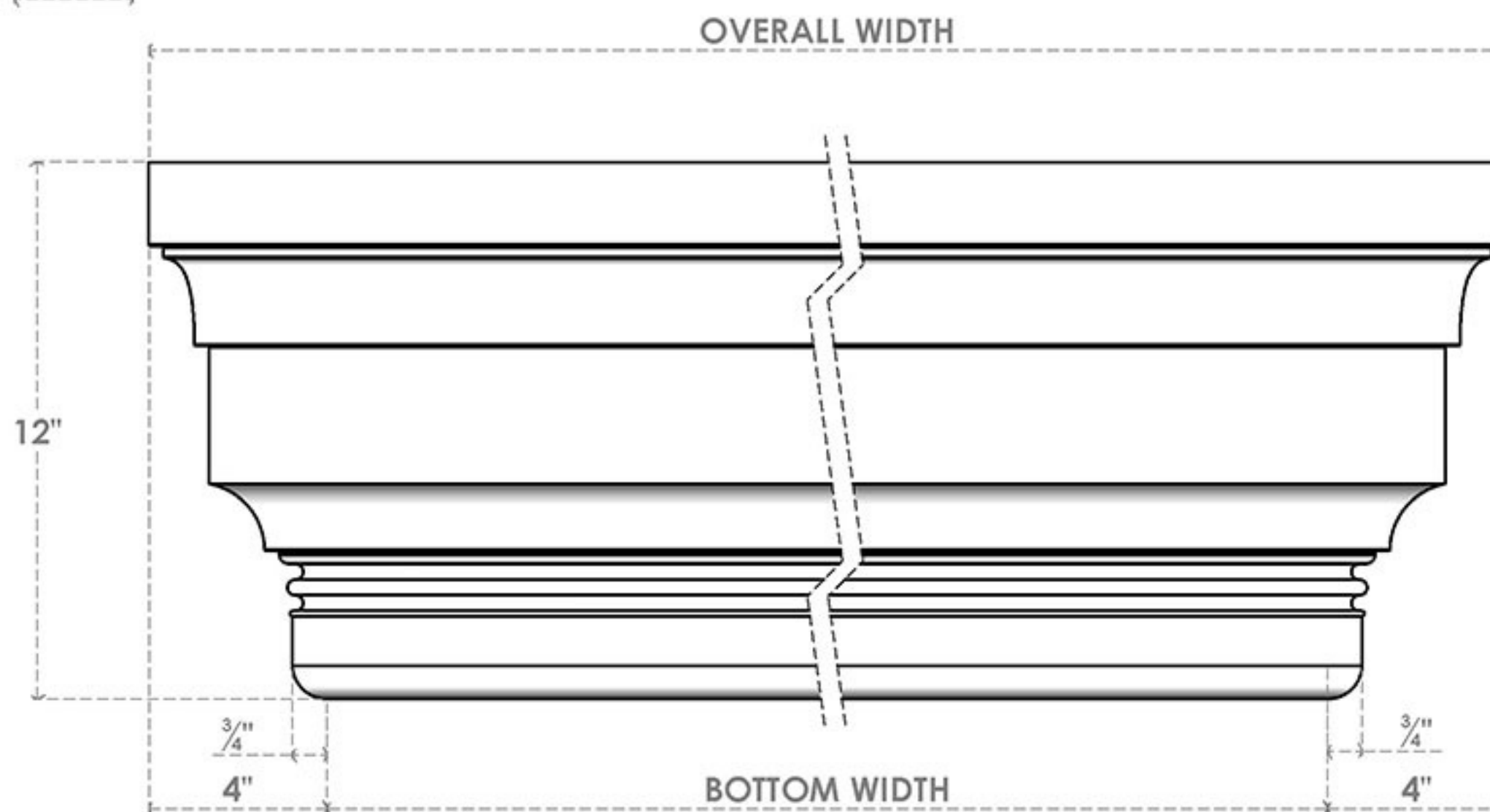
FRONT
