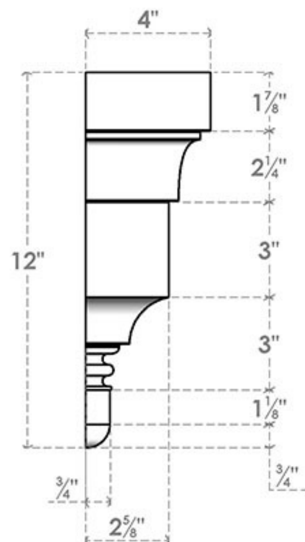
SIDE
