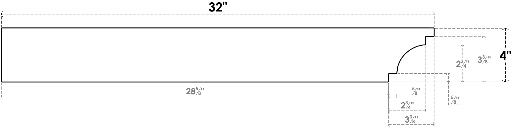
SIDE PROFILE
