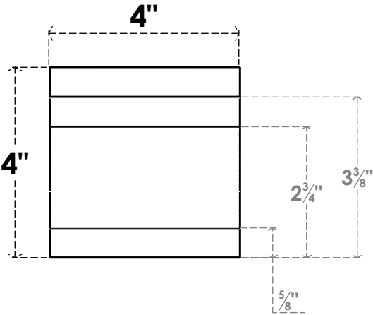
FRONT PROFILE
