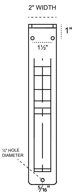
FRONT PROFILE
