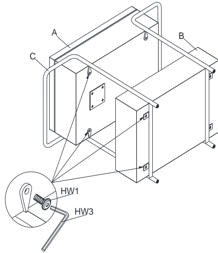
STEP1 assemble the metal frame and the body
