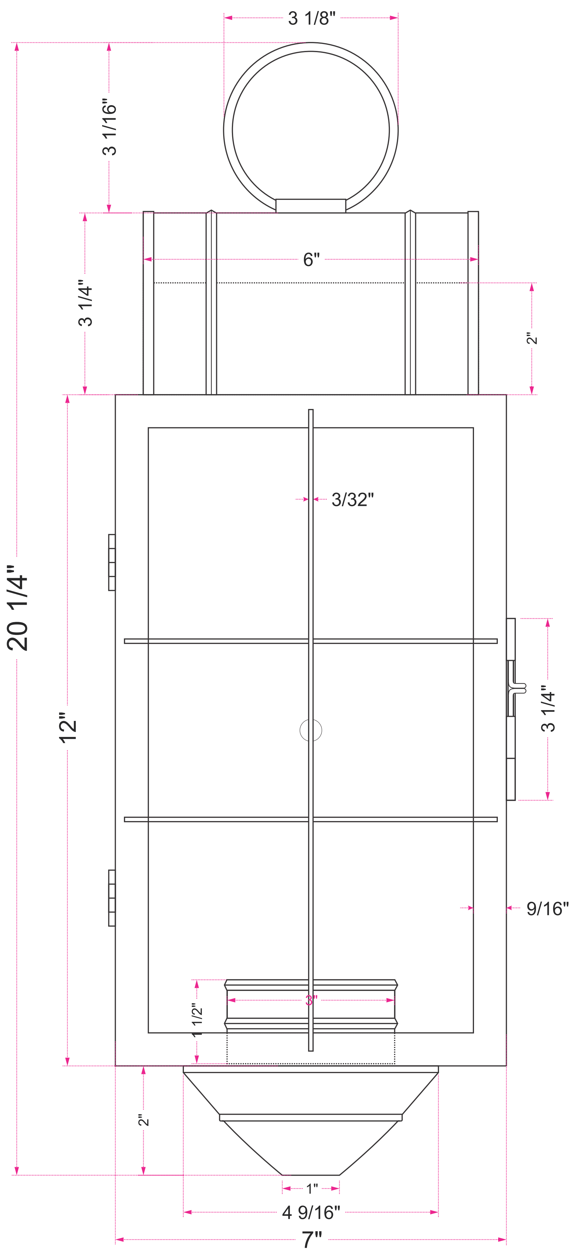
Front View
