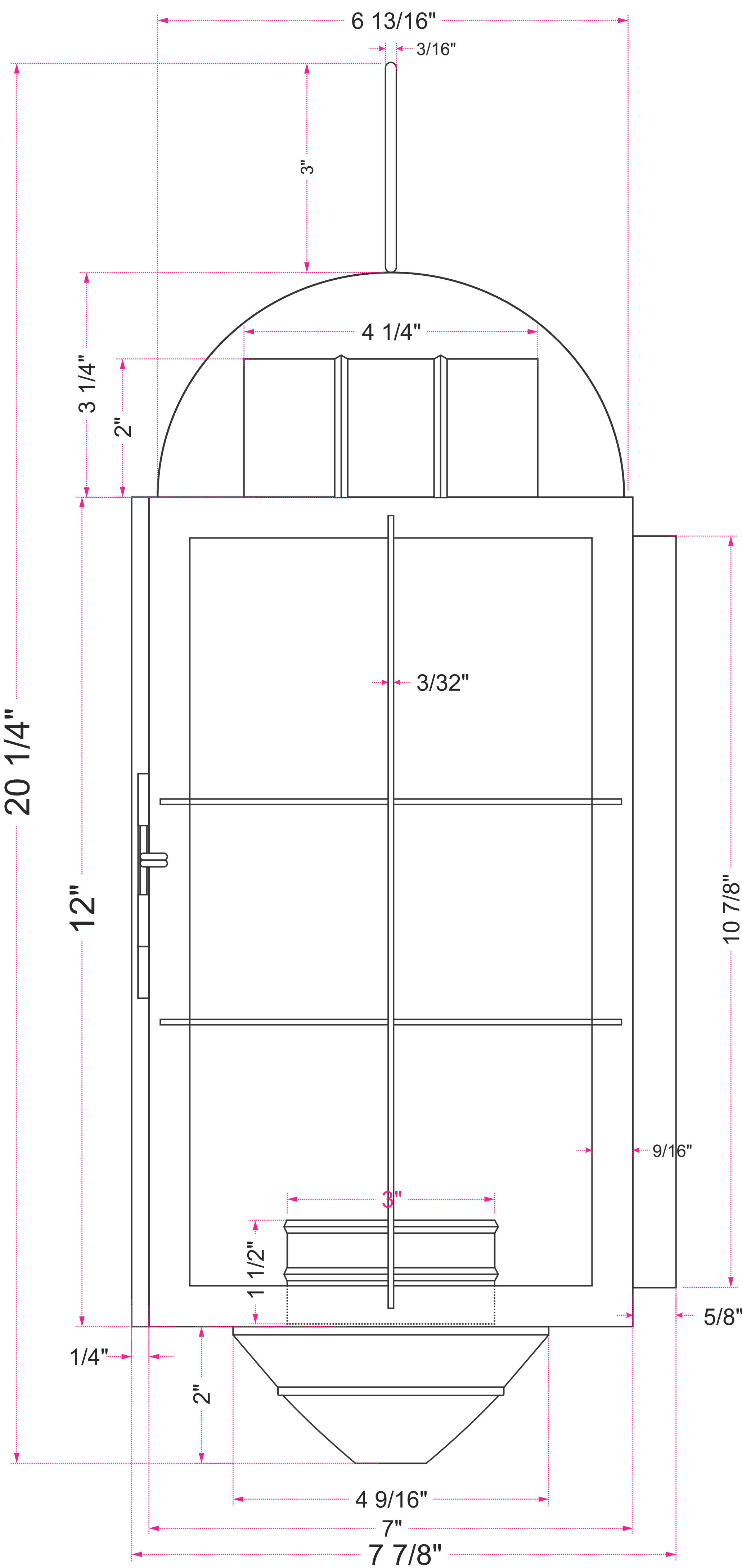
Side View
