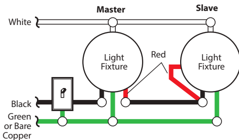
Wiring Diagram 2
