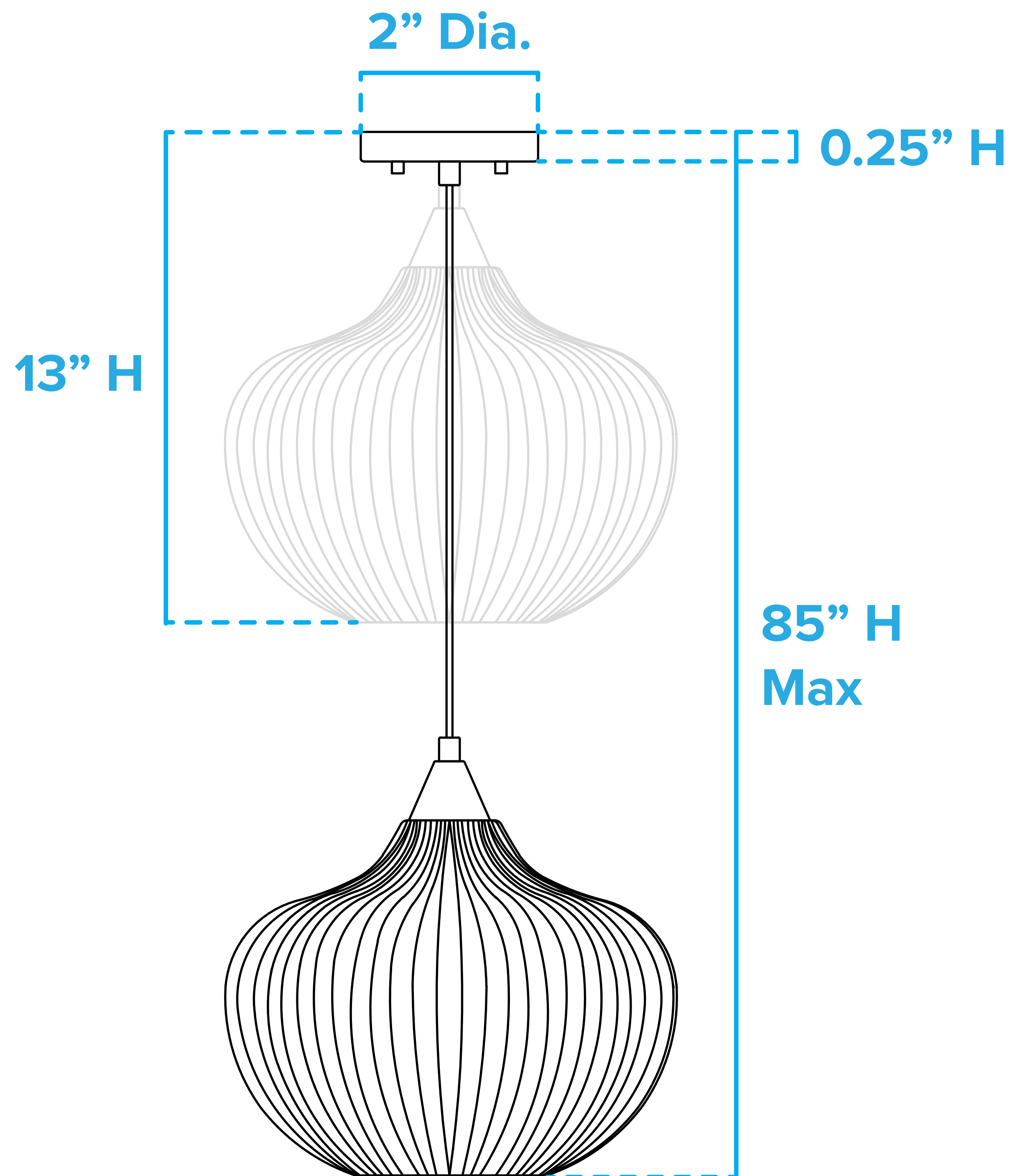
Front View
