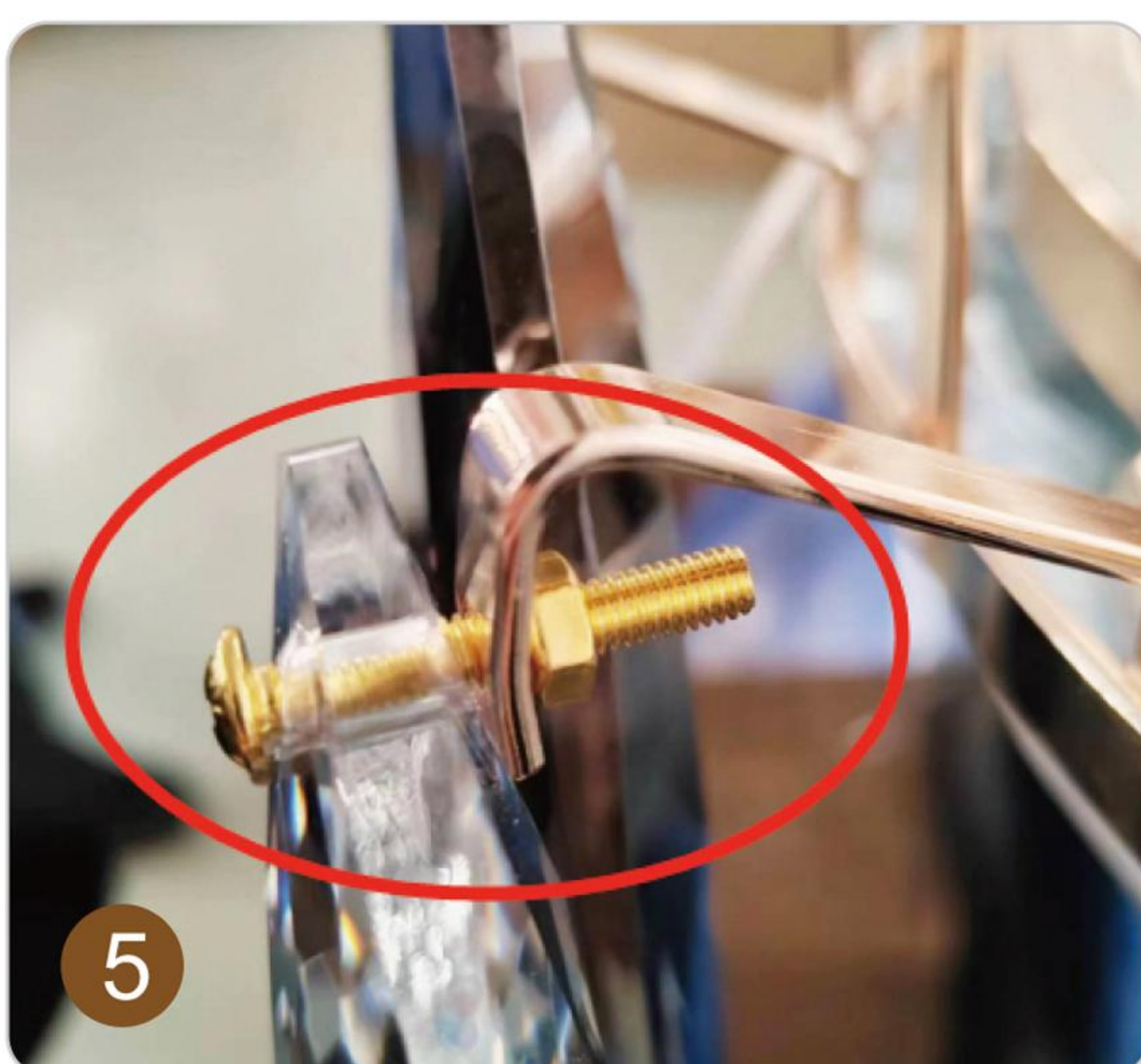
⑤The screw goes through the crystal and is fixed in place by the lamp holder and the lock nut.
