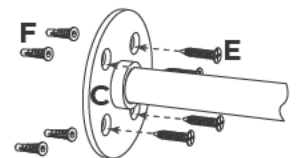
Option B For drywall
