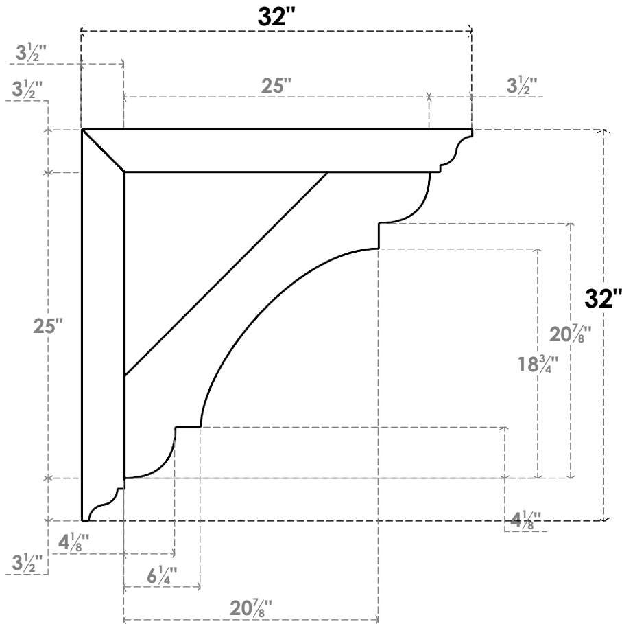
SIDE PROFILE
