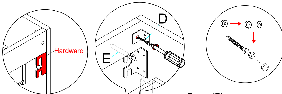
Screw (D): M5 x 50mm long (2pcs)
