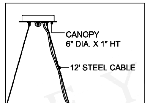
CANOPY DETAIL
