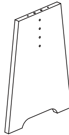
31 (400*297*18mm x2)
