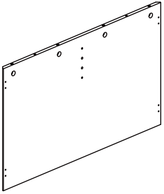
21 (660*400*12mm x1)
