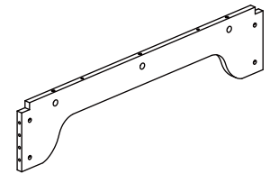
32 (800*170*15mm x1)
