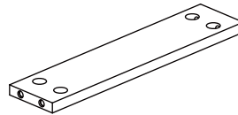
11 (290*60*12mm x3)
