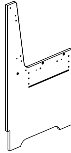
3 (870*500*15mm x1)
