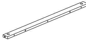
7 (688*40*15mm x1)
