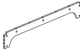
27 (930*145*15mm x1)
