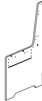
4 (870*500*15mm x1)
