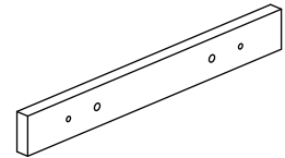
12 (283*35*12mm x4)
