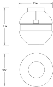
DFI12 GARRISON FLUSH MOUNT
