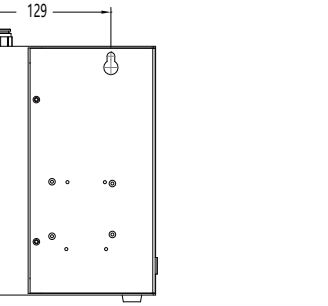
(Dimension of punching (mm)) (Diagram of Wall-mounted Installation)
