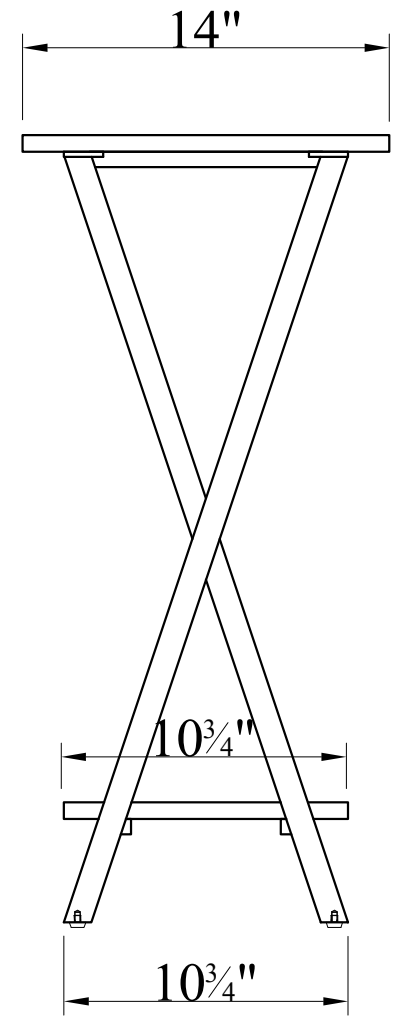
SIDE VIEW
