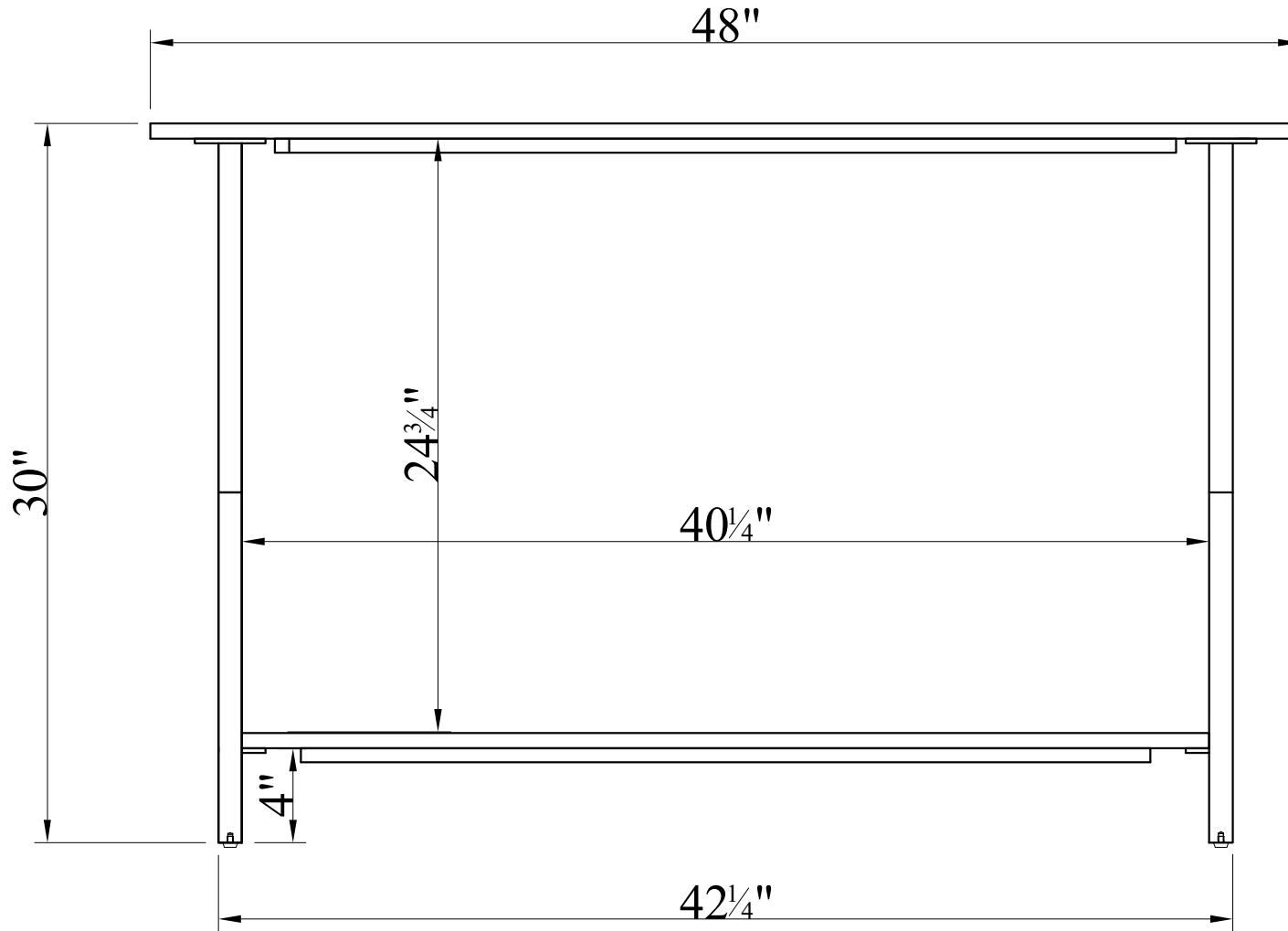
FRONT VIEW
