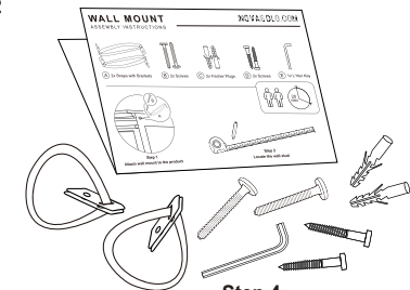
Step 4 Install the Wall Mount per the Wall Mount - Anti-Tip Kit assembly instructions.
