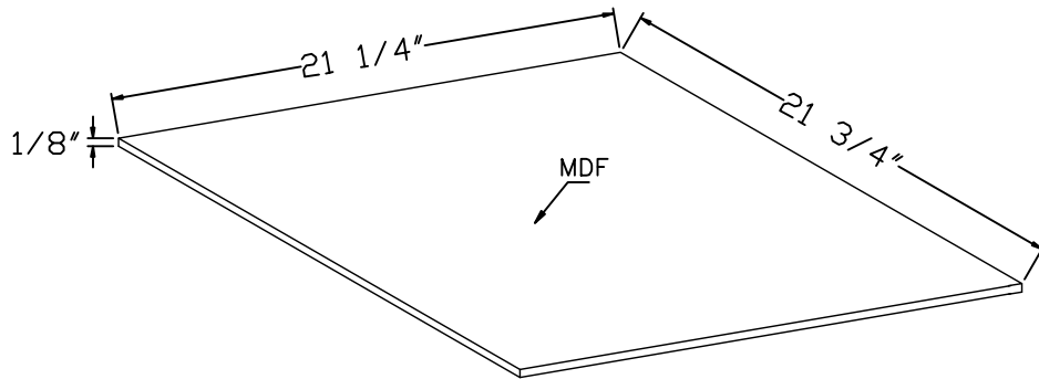
DRAWER BOARD
