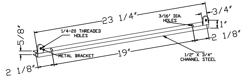
SUPPORT RAIL
