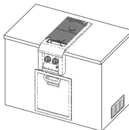
TYPICAL ISLAND INSTALLATION (AEB122 SHOWN)
