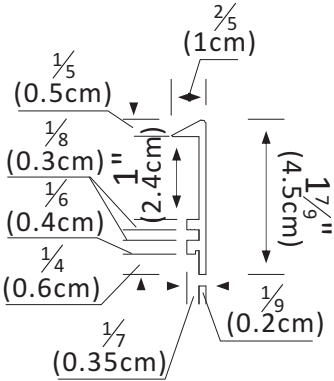
Aluminum section
