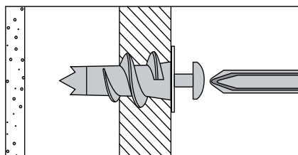
2. Plasterboard Wall Plug
