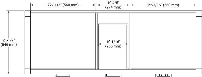
PLAN VIEW
