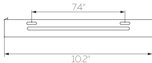
UPPER BRACKET
