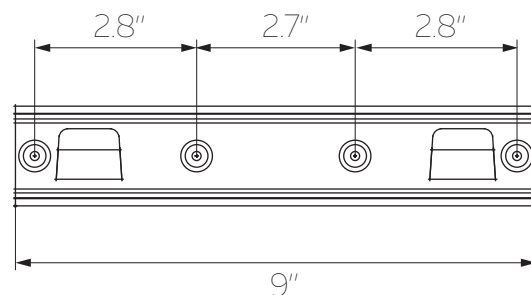
LOWER BRACKET
