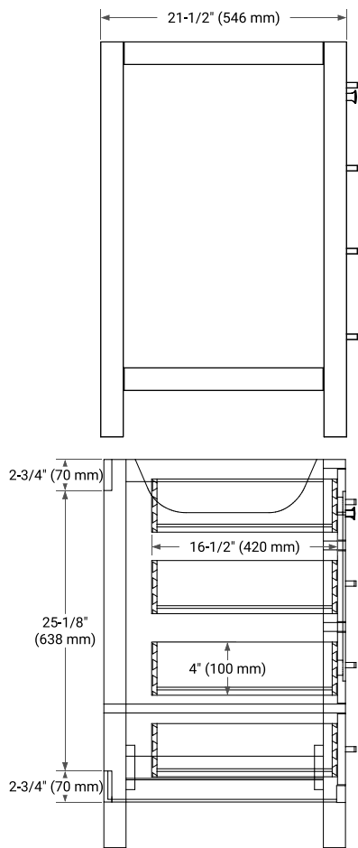
SIDE VIEW
