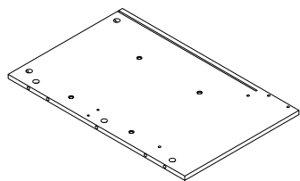
1 (580X375X12mm)X2
