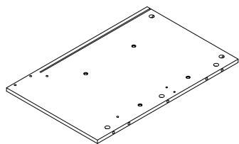
2 (580X375X12mm)X2
