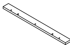
3 (580X50X15mm)X2
