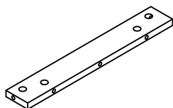
19 (334X50X15mm)X2
