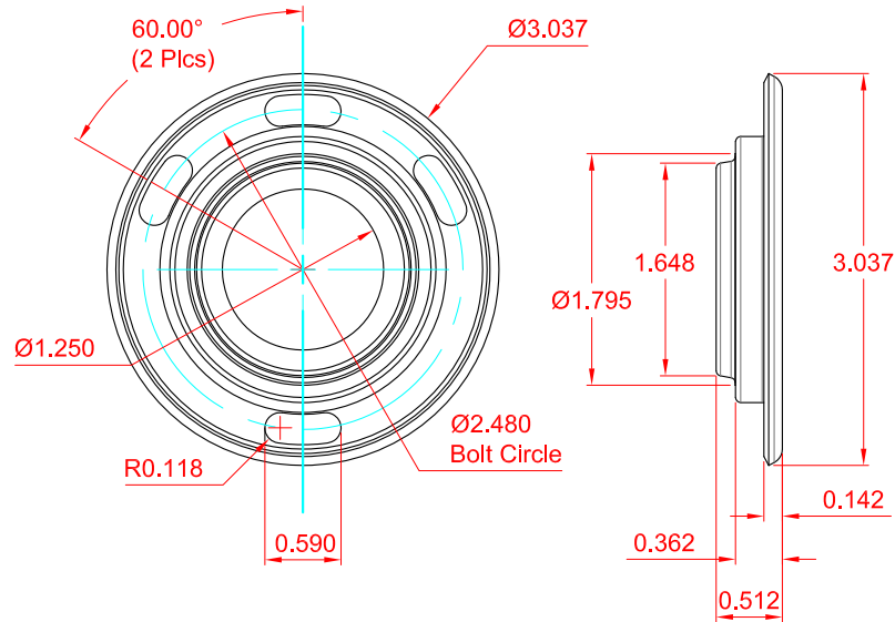
IFSS-CER-FLANGE Detail
