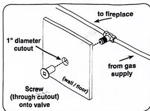
Fig. 3-1 Gas valve orientation
