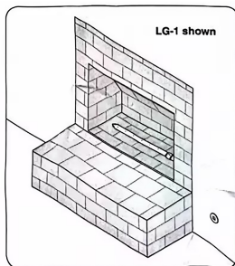
Fig. 3-3 Install log lighter in fireplace
