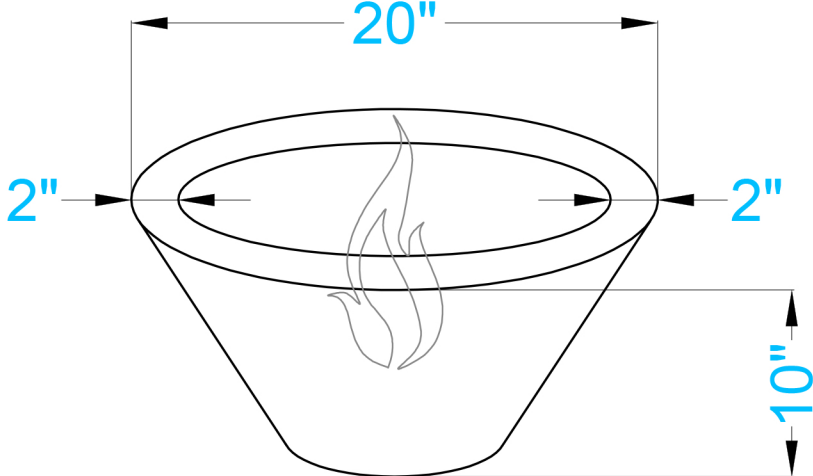
AXONOMETRIC VIEW
