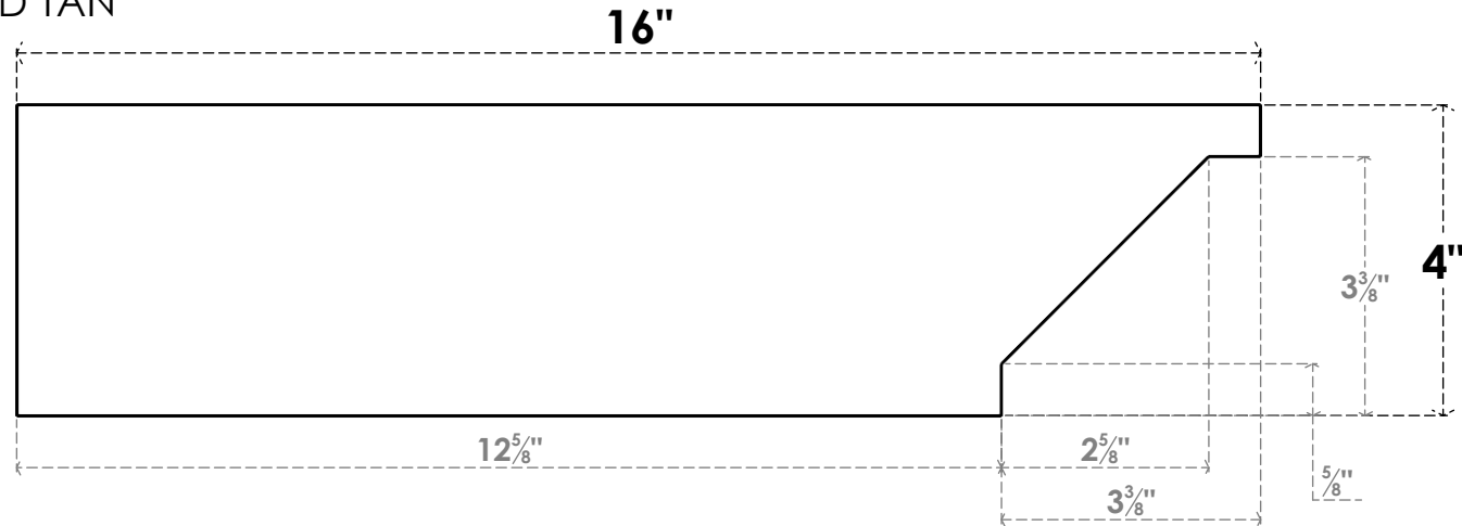
SIDE PROFILE
