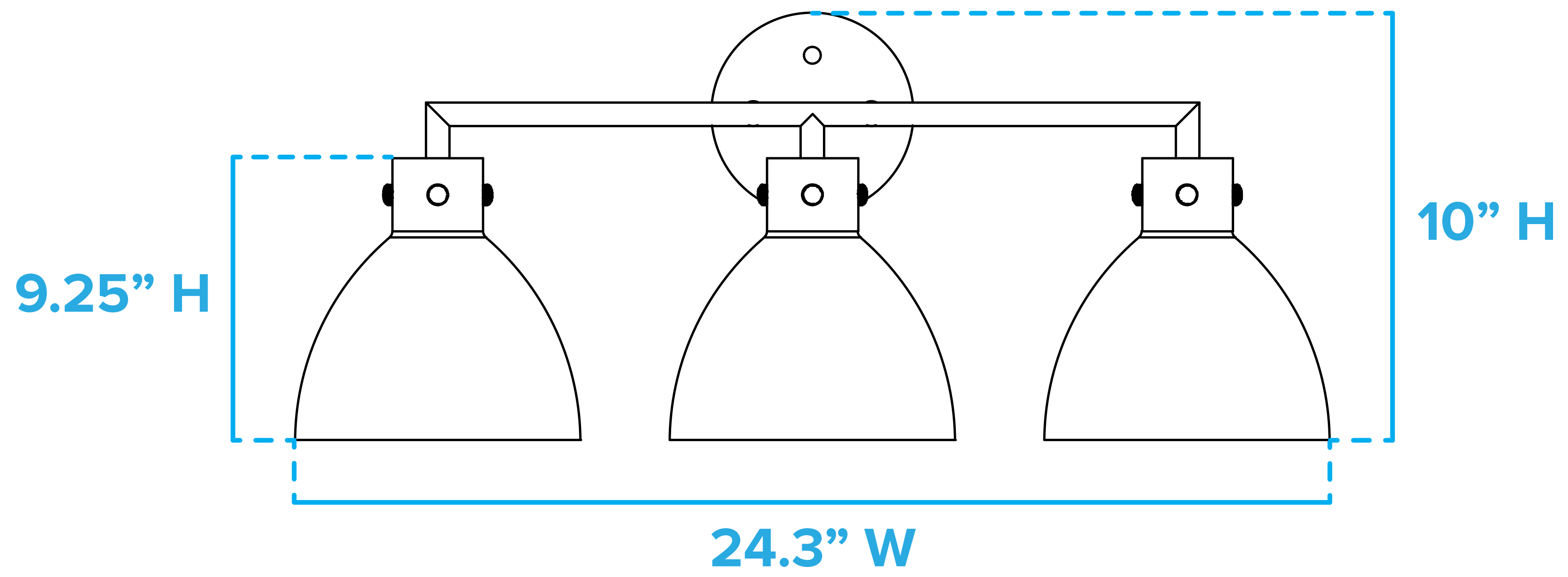
Front View
