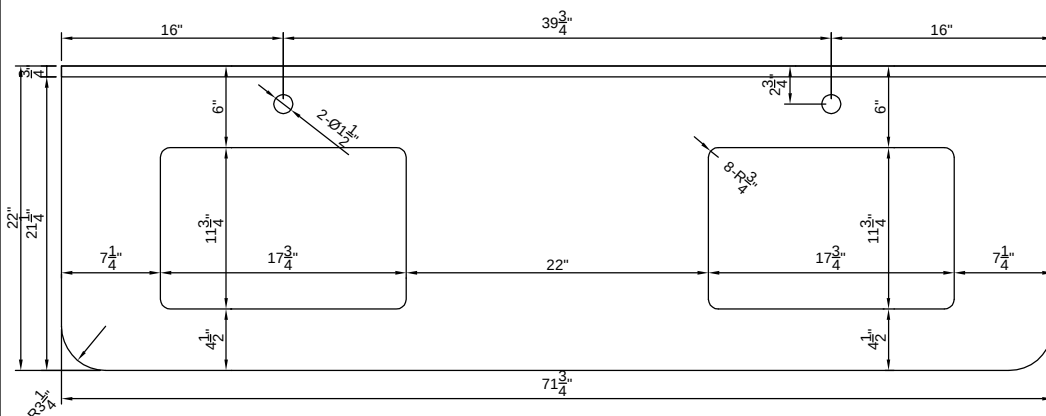
TOP VIEW OF VANITY CABINET
