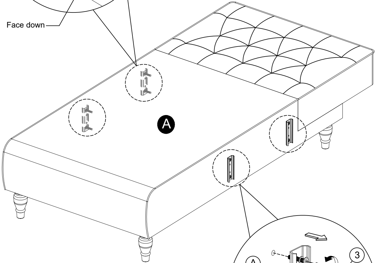
Female Bracket Joint
