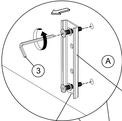
Male Bracket Joint
