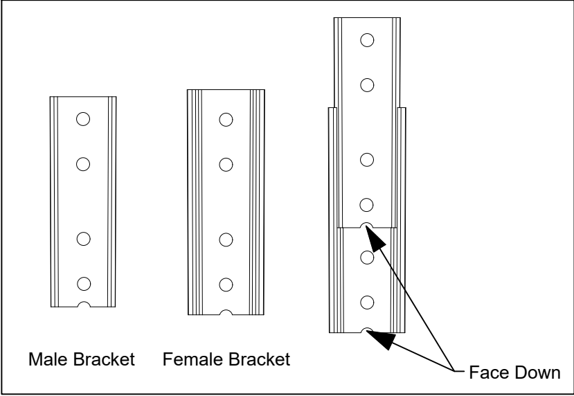
Male Bracket Joint
