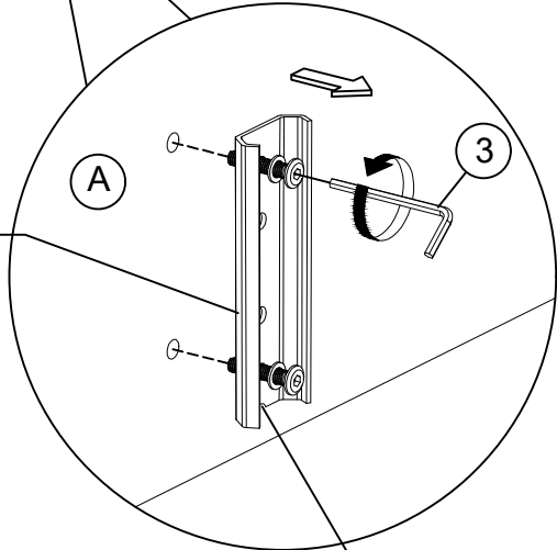
Female Bracket Joint
