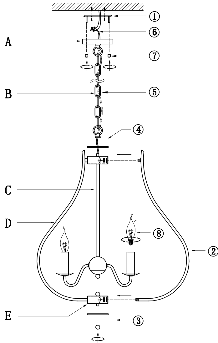
Installation sequence diagram
