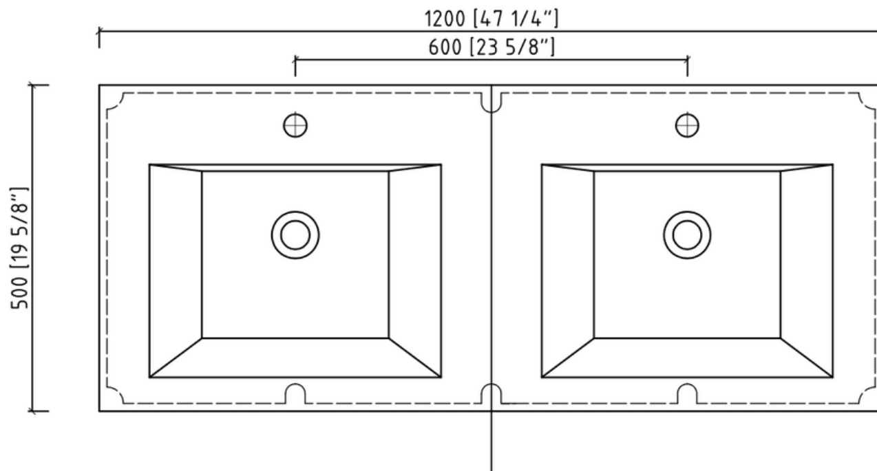
SECTION B-B
