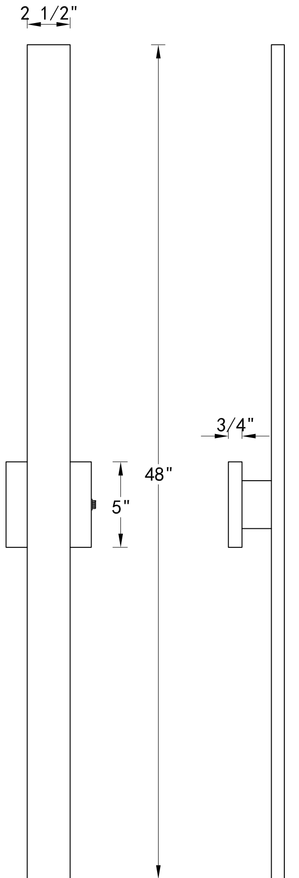
FRONT VIEW
