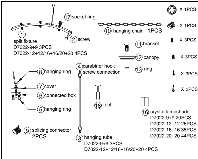
1.Combine the split light fixture together and fasten it with screw ②.
