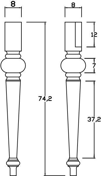
LEG DETAIL
