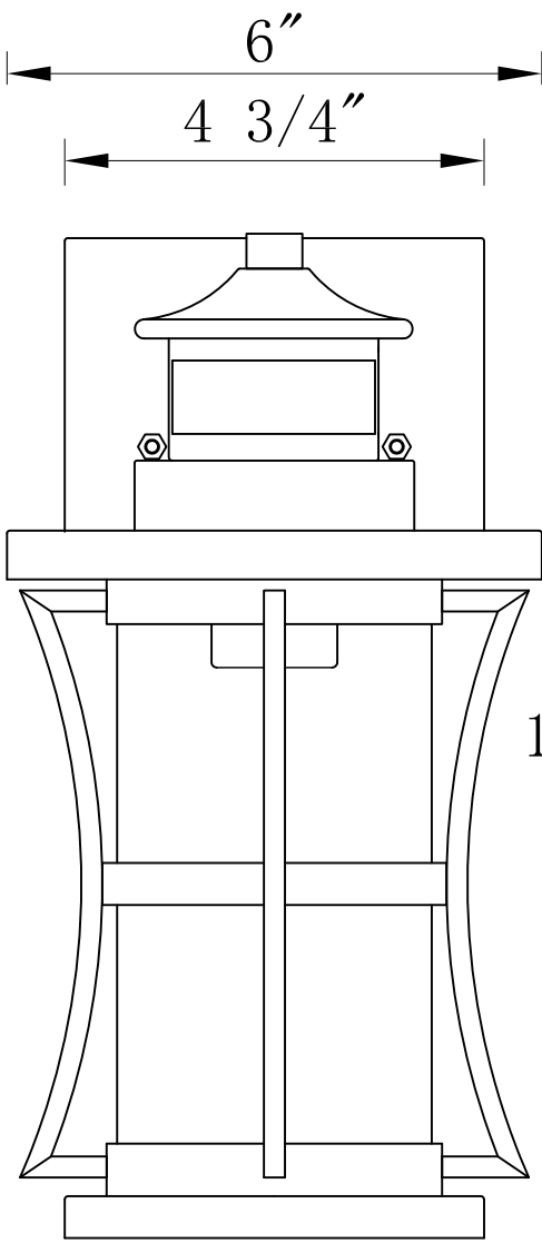
FRONT VIEW
