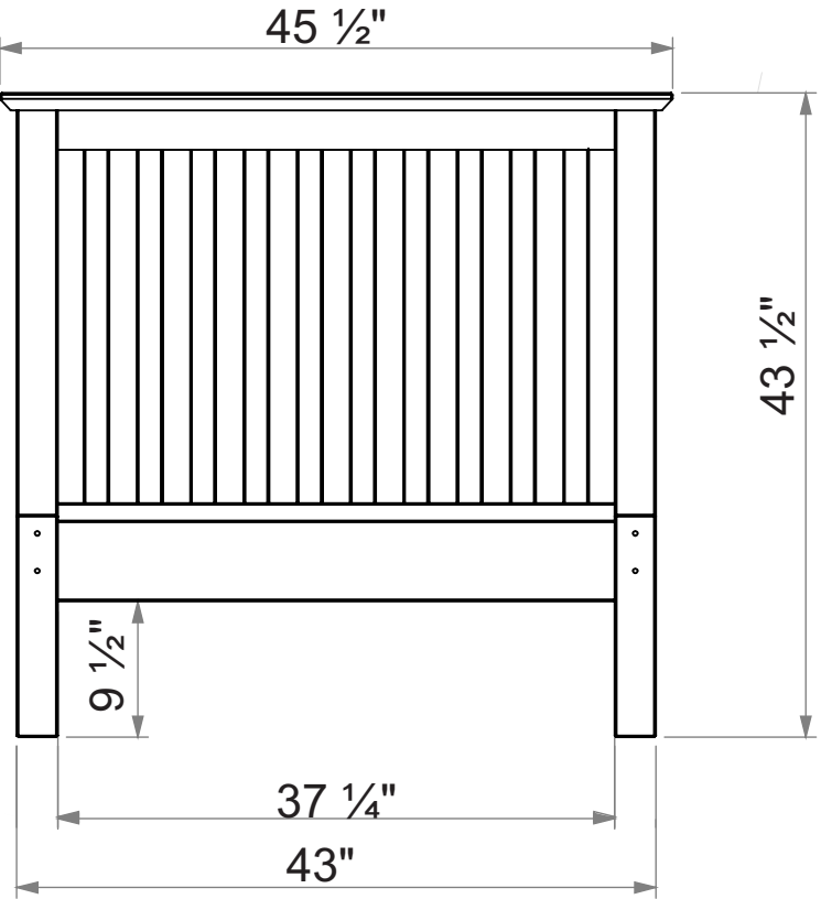
Frontal View
