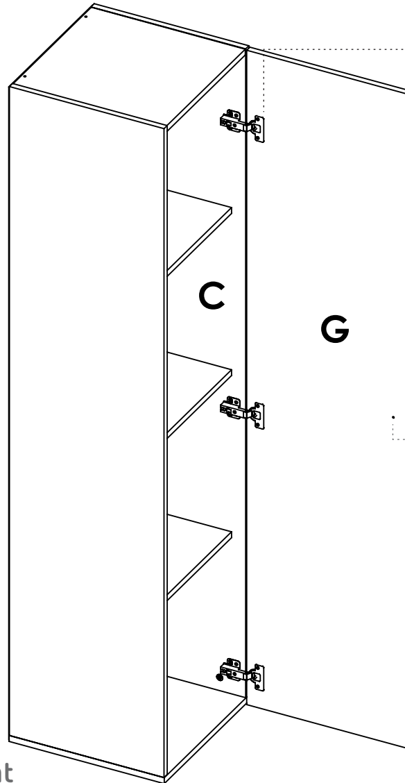
Hinge adjustment
